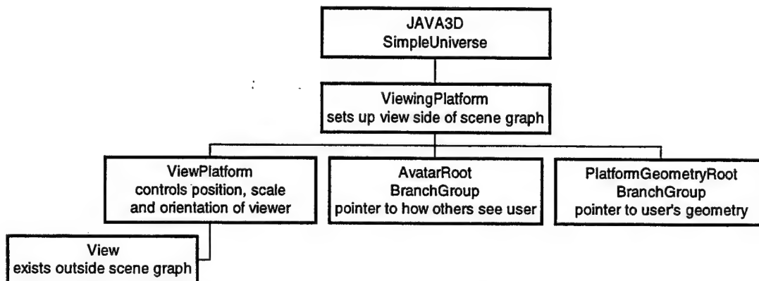
Figure 5.3. ViewingPlatform hierarchy.
